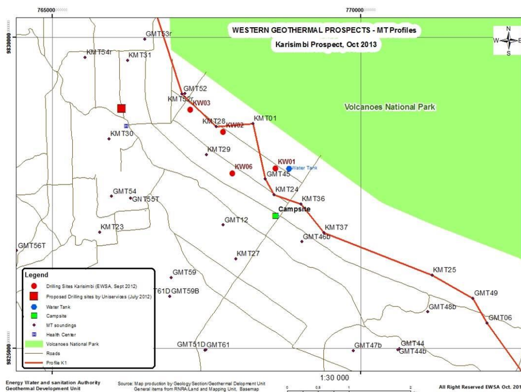
Figure 3: Location of wells in Karisimbi prospect (GDU, 2013)
